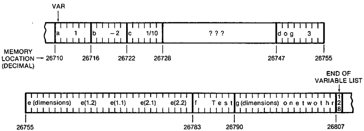
Fig. 3-8. Typical variable list.
